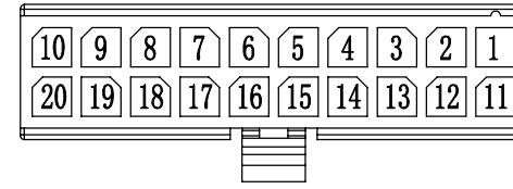
20-Circuit Housing
