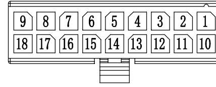
18-Circuit Housing
