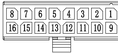
16-Circuit Housing
