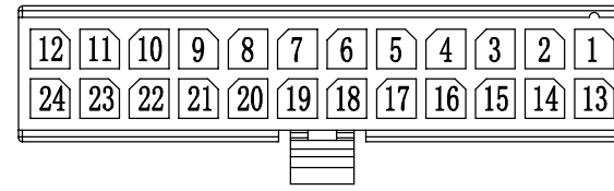
24-Circuit Housing
