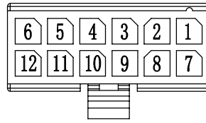
12-Circuit Housing
