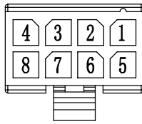
8-Circuit Housing
