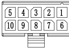
10-Circuit Housing
