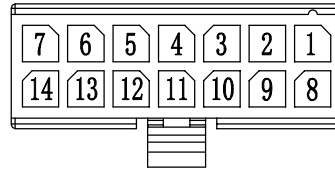
14-Circuit Housing
